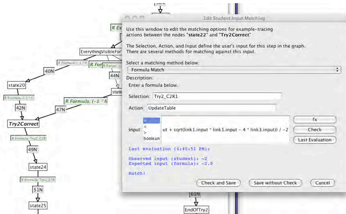
Fig. 23. Dialog box for attaching a formula to a link; the formula expresses how the value on the link depends on values on other links.
