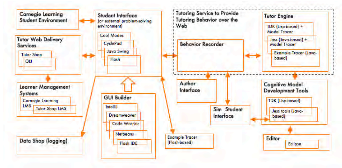
Fig. 25. CTAT's modular architecture.
