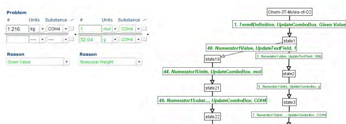
Fig. 16. Demonstrating the first steps of an alternative, correct solution.
